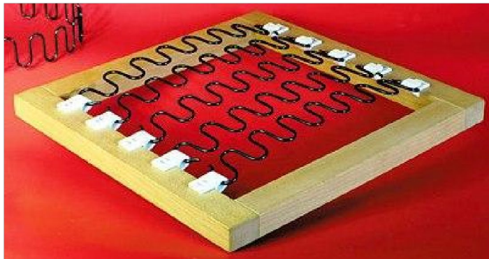
Picture 5.10: Zigzag arch hinge
