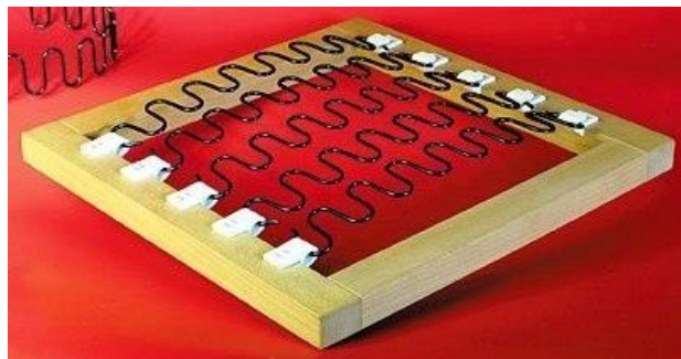
Picture 3.8: Furniture frames hammered zigzag arch
